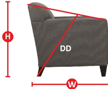
Sofa diagonal depth DD must be less than the entryway dimensions 2 , stairway dimensions 3 , 4 , & 8 , and all interior doorways 6 or 7
